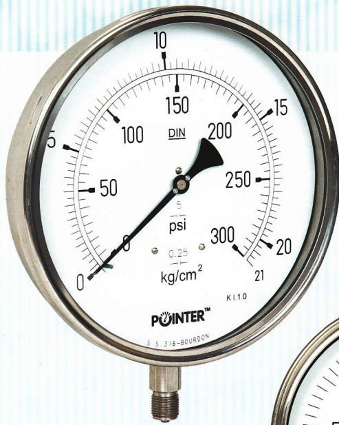
250mm Bottom Mounting
